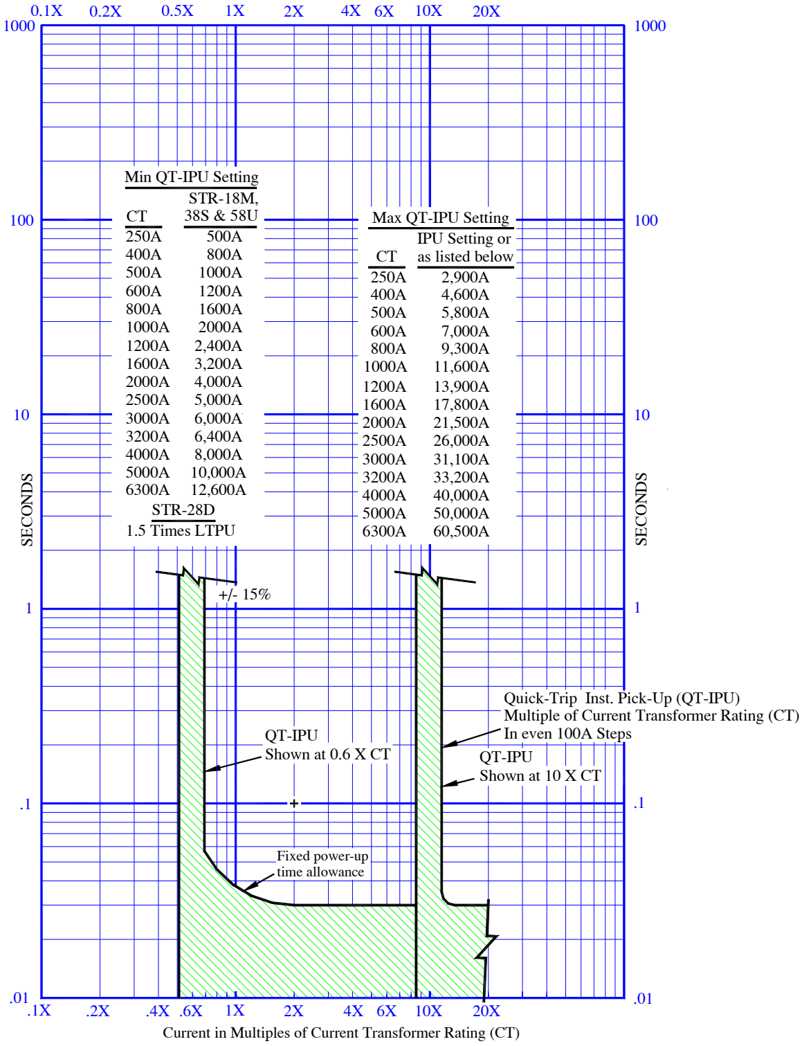
AC-PRO-MP Quick-Trip™ Instantaneous Time Current Curve
